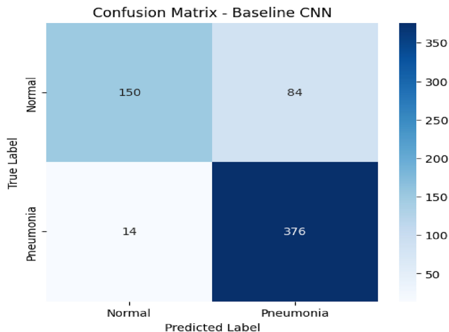
FIGURE 8 | Confusion matrix - baseline CNN.
